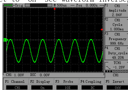
Figure 2-7 waveform inverse
