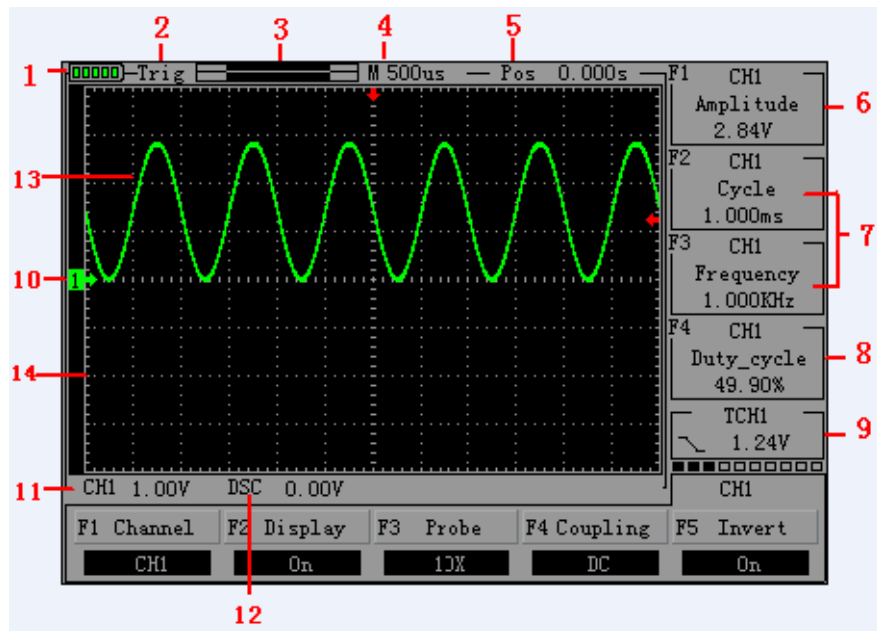
Figure 1-2 screens
