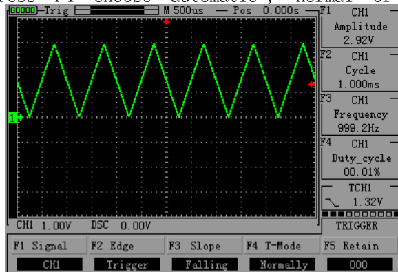
Figure 2-15 normal trigger
