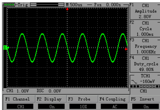
Figure 2-5 coupled ac
